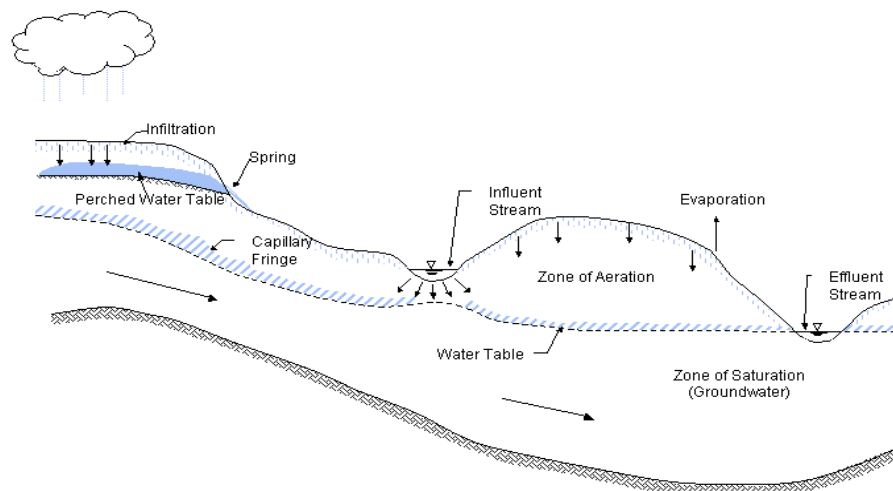
Figure 6-3: Schematic Illustration of the Occurrence of Groundwater in an Unconfined (Water Table) System (Adapted from FHWA, "Highway Subdrainage Design")
