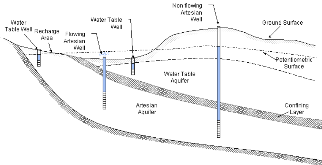
Figure 6-4: Confined Aquifer (artesian flow conditions) Adapted from FHWA, "Highway Subdrainage Design"
