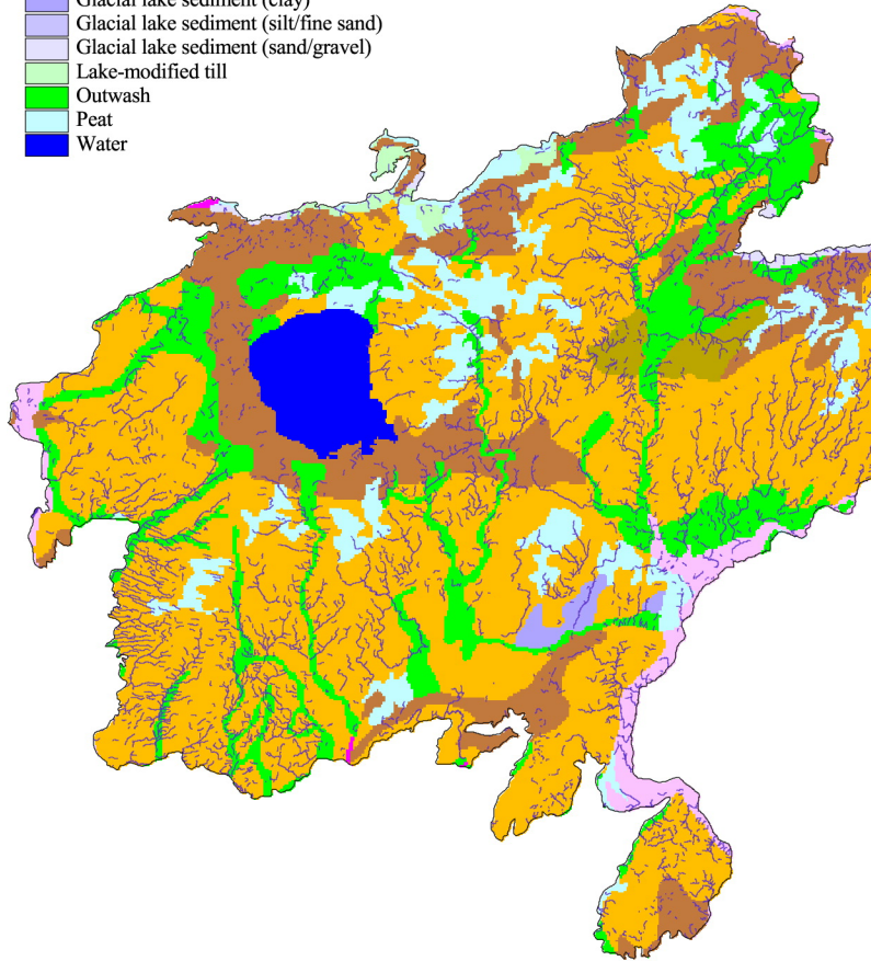
Generalized Quaternary Geology
