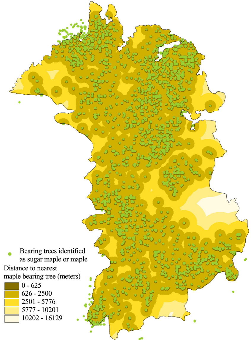
Distribution of Sugar Maple
